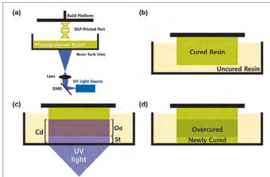
Figs 1a-d DLP: the structure of the DLP printer and the overcuring mechanism of the photosensitive material during the lamination process. (a) A schematic representation of a bottom-up DLP printing process. (b) Printing state before UV irradiation for adhesion of a new layer. (c) As UV light penetrates to cured depth (Cd), the uncured fresh resin undergoes curing, whereas the already cured resin undergoes additional polymerisation, or "overcuring", where the overcured depth (Od) is determined by the UV light energy, resin absorption coefficient and slice thickness (St). (d) Successful adhesion of a new layer as a result of sufficient crosslinking between the layers due to the overcuring effect. (Reprinted from Lee et al 51 with permission.)
