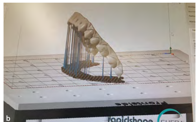
Figs 9a-b Production procedure for Graphy direct aligners. Support pins were added in Rapid Shape Netfabb software (Heimsheim, Germany). The layer thickness was 0.5 mm.
